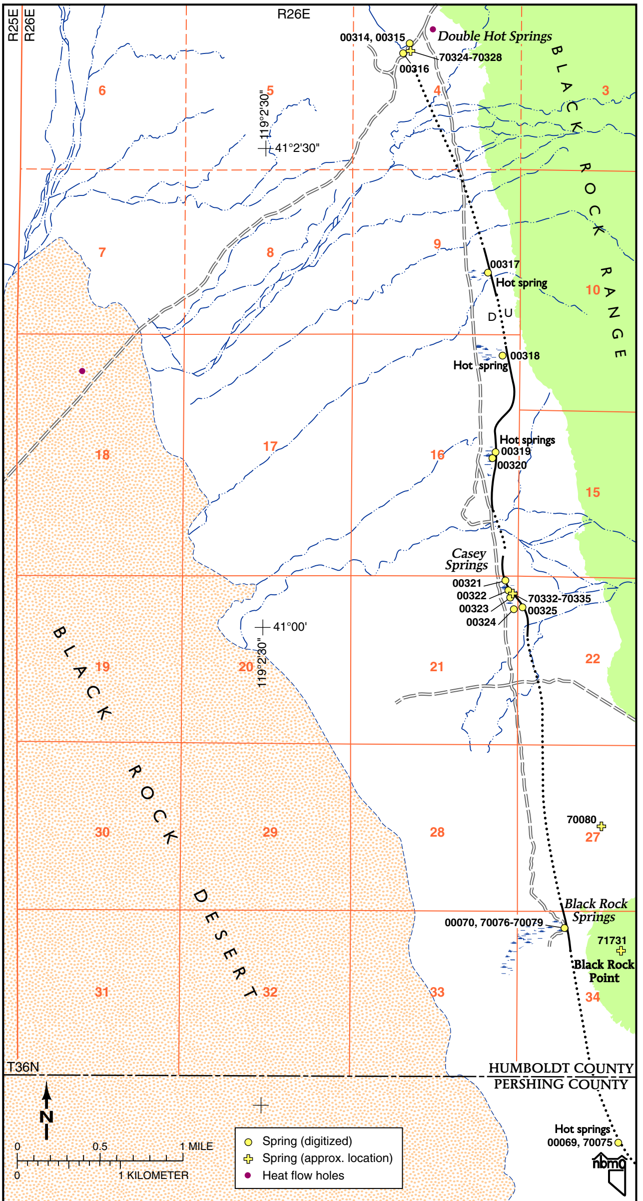
Double Hot Springs and Black Rock Point West Quadrangles
